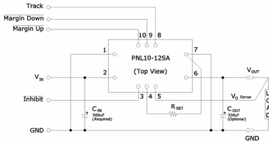
Figure 1 Circuit configuration for programming output voltage
